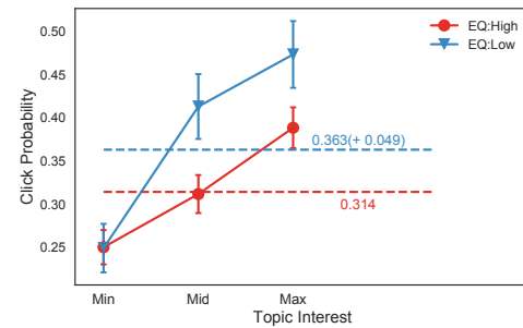
Figure 6: Click probability of the news with different levels of quality and user topic interests.
