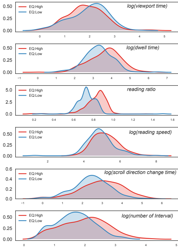
Figure 7: The probability density function (estimated by kernel density estimation) of behaviors when users are reading the news of different qualities (EQ:High vs. EQ:Low)
